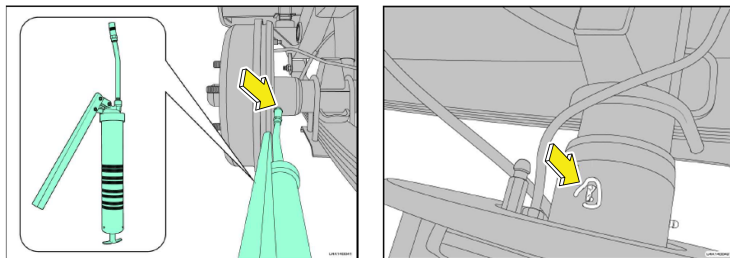
Rear Axle Housing (LH & RH)
