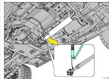
Prop Shaft Sliding Yoke (F & R shafts)
