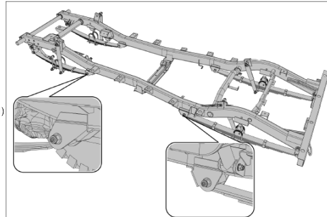
Front Leaf Spring Pivot End (LH & RH)
